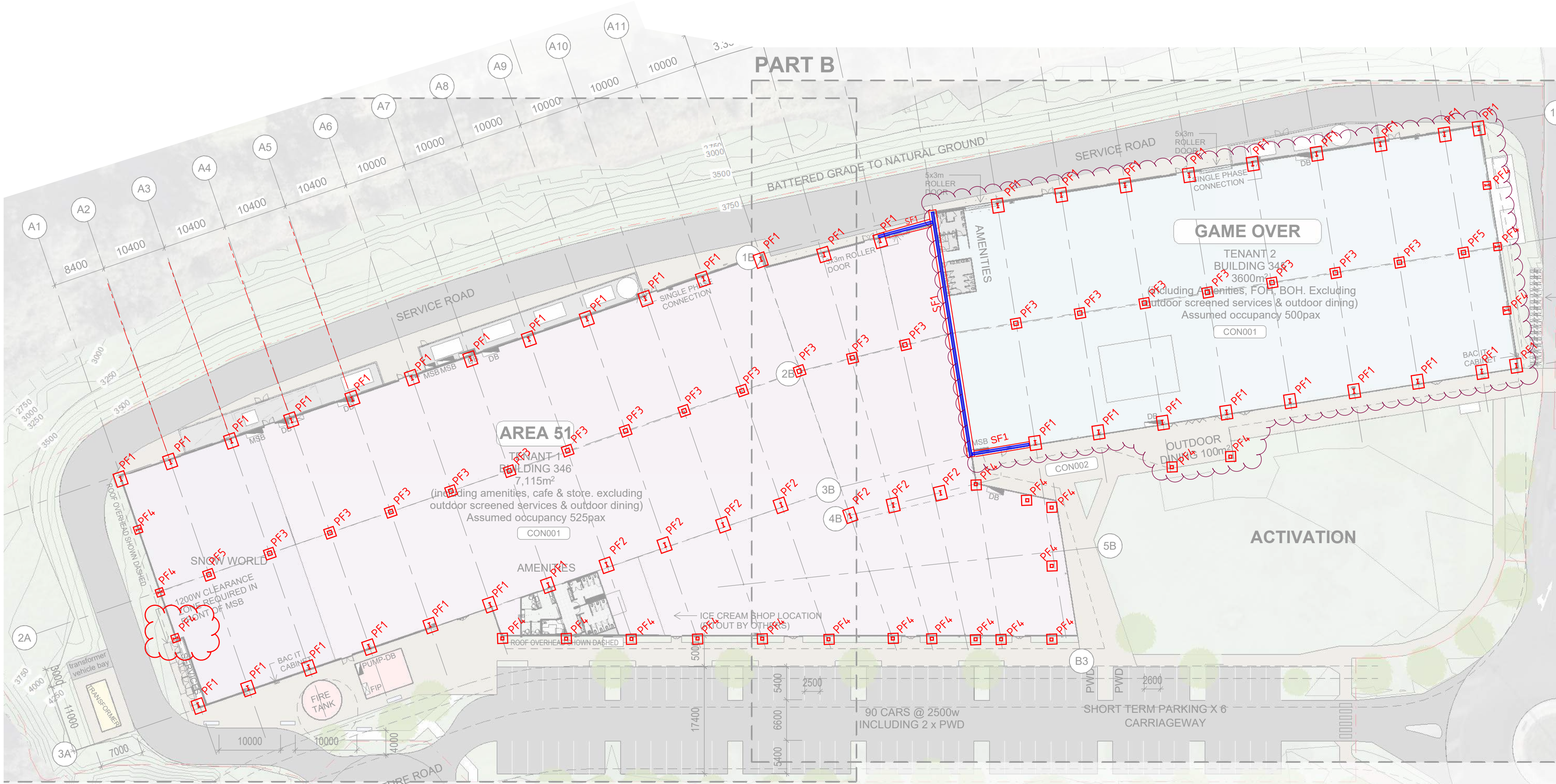
FOOTING PLAN
